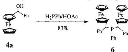
Scheme 2. Synthesis of Bis(ferrocenylmethyl)phosphine 6
